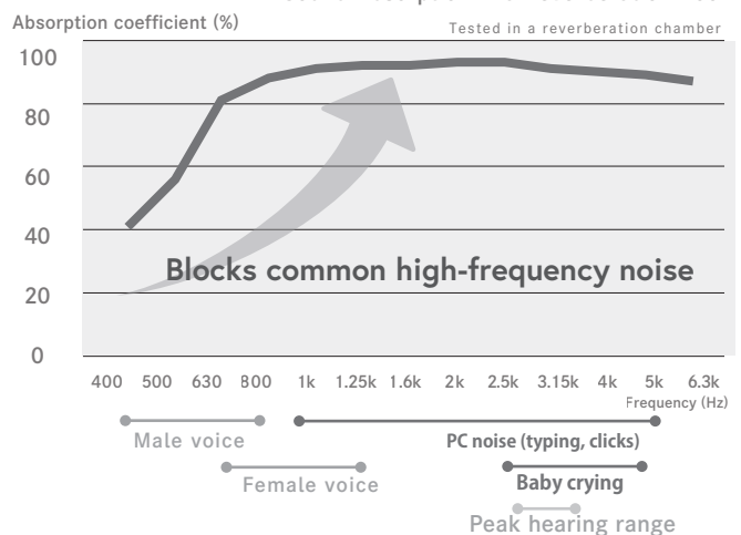
Sound Absorption in a Reverberation Room
